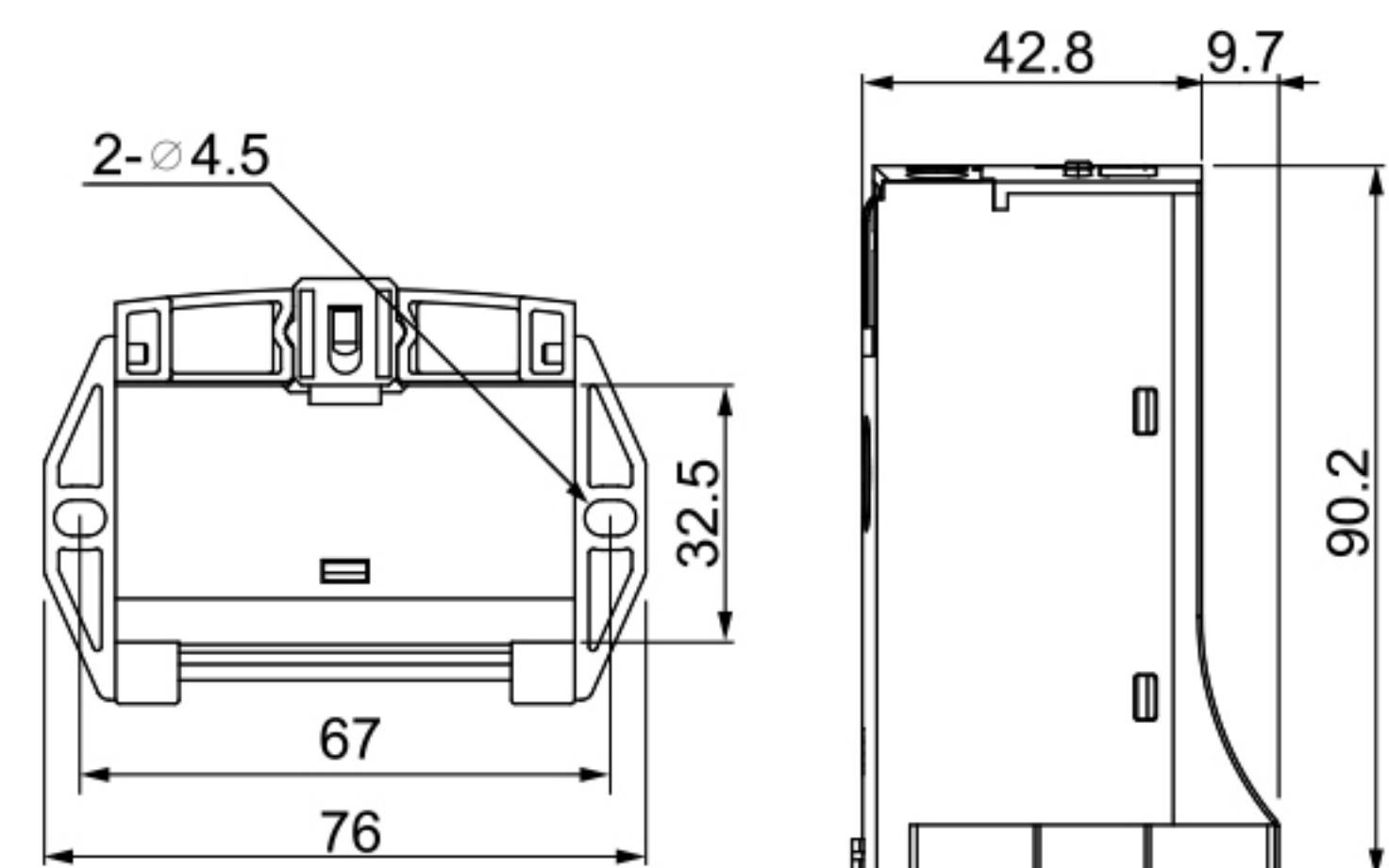
DIN Rail & MOUNTING HOLE SIZE
