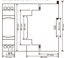
Dimensions for FKV-11/12
