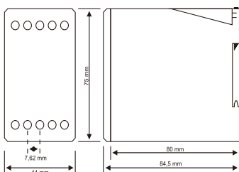
Dimensions for FK-01/02
