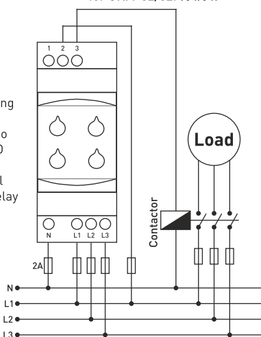
Connection Diagram for GKM-02/02F/04/04F
