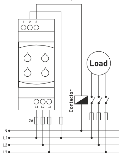
Connection Diagram for GKT-03/03F/05/05F
